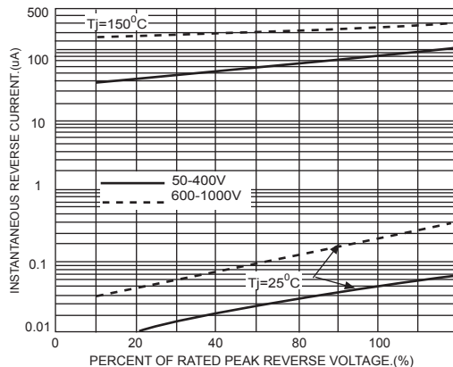
FIG.4-TYPICAL REVERSE CHARACTERISTICS PER BRIDGE ELEMENT(GBU6005 THRU GBU810)
