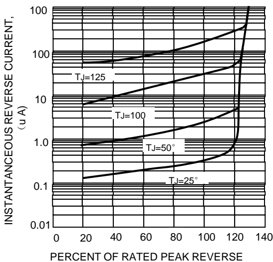
FIG.5-TYPICAL REVERSE CHARACTERISTICS
