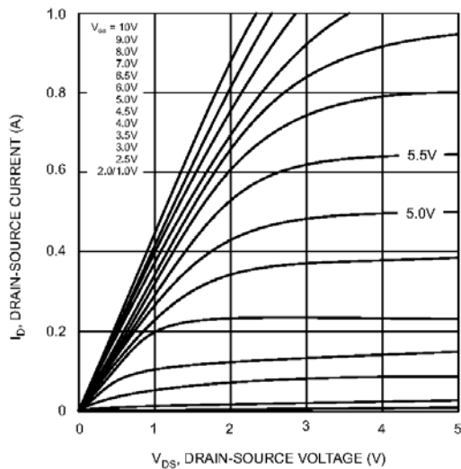
V DS , DRAIN-SOURCE VOLTAGE (V) Fig. 1 On-Region Characteristics
